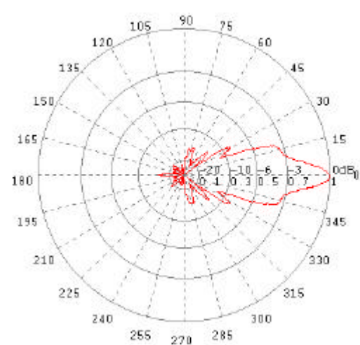
H-Ebene / H-Plane 4 GHz
