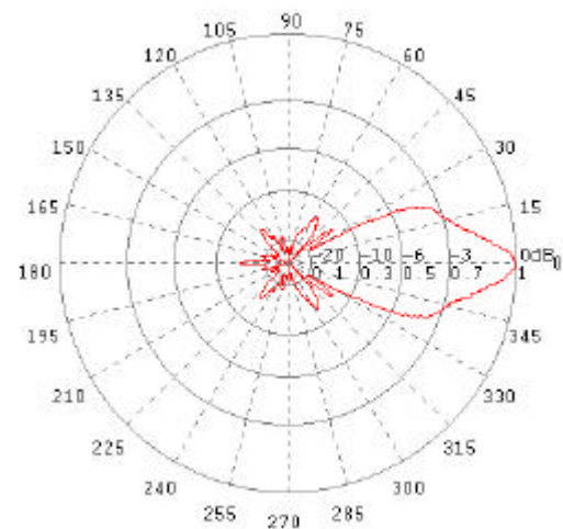
H-Ebene / H-Plane 3.5 GHz
