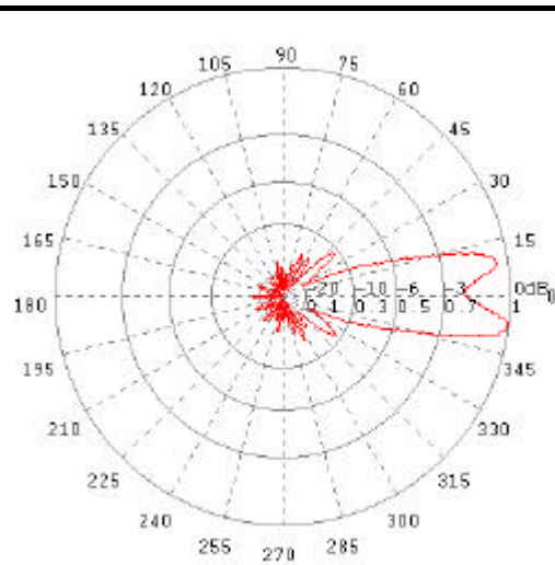
E-Ebene / E-Plane 4.5 GHz
