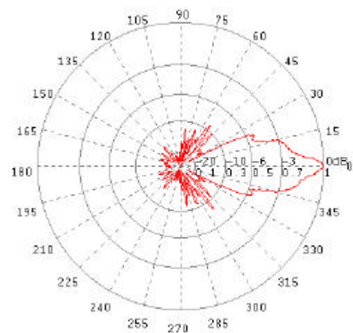
H-Ebene / H-Plane 5 GHz
